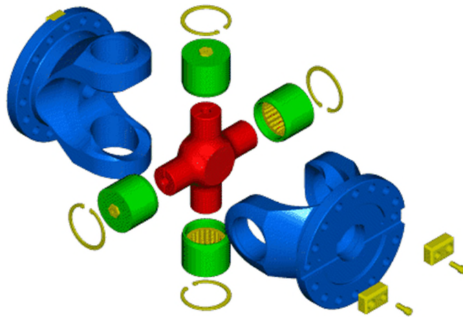
Figure 3-9, Universal Joint Exploded View
