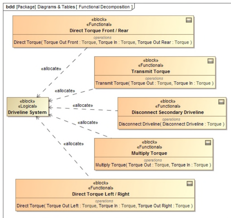
Figure 2-1, SysML Driveline Functional Decomposition
