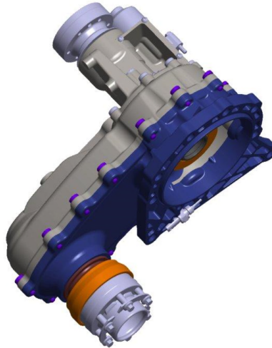
Figure 3-4, Transfer Case
